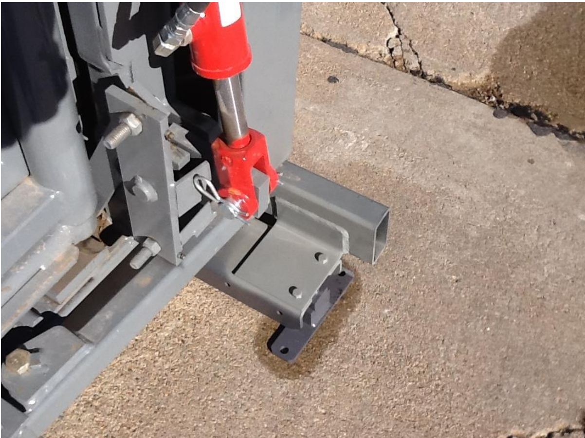
Chuteweight bars on a Silencer Chute
